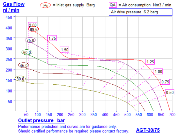
AFP-GB-01-15K AGT-30/75 Pump performance curve
