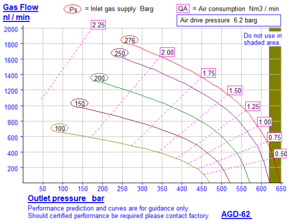
AFP-GB-01-05K AGD-62 Pump performance curve
