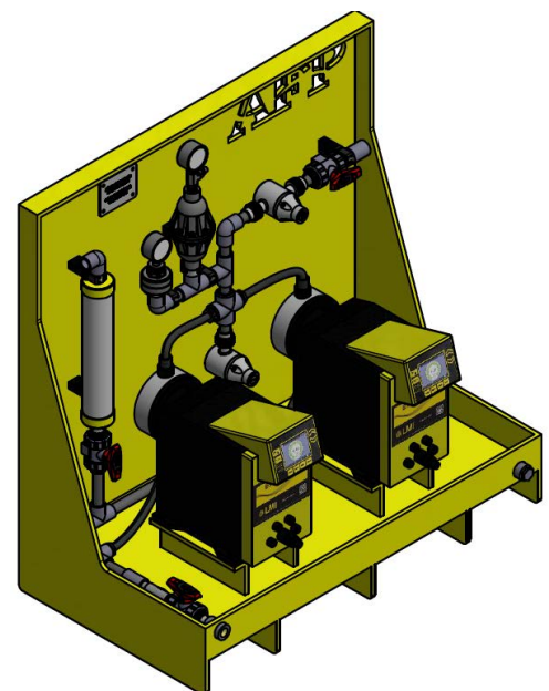
DOSU-D Double pump design
